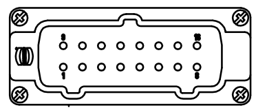
HARTING CONNECTOR 1 :
